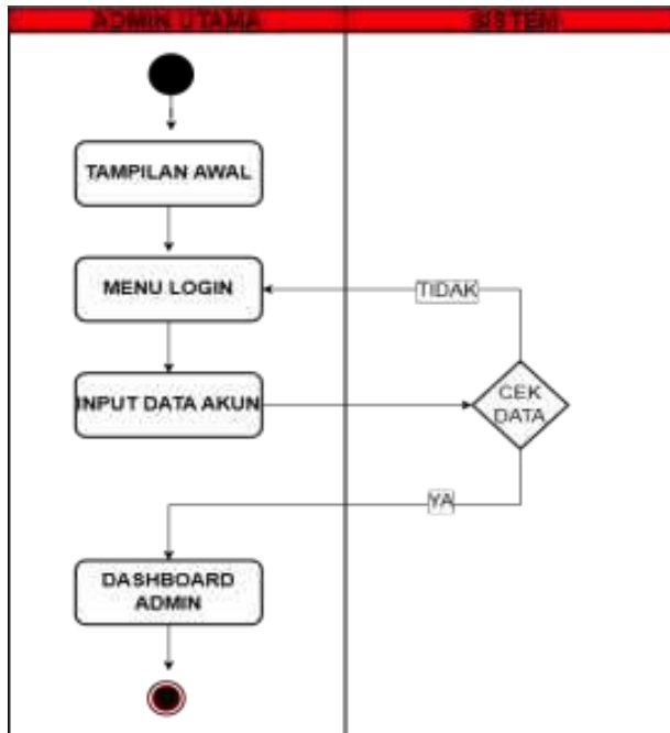
Gambar 3: Activity Diagram
