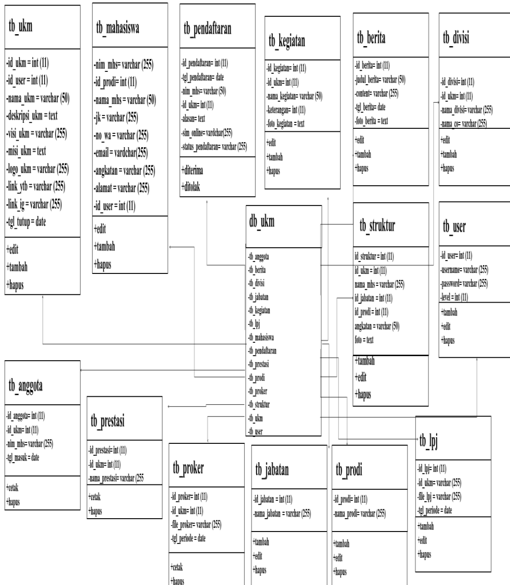
Gambar 2: Class Diagram
