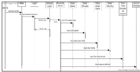
Gambar 5. Sequence Diagram Pengelola
