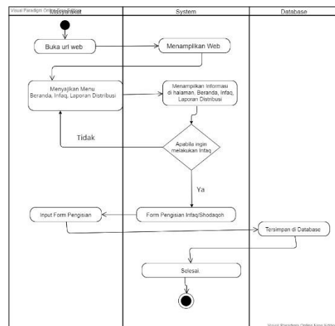
Gambar 4. Activity Diagram Masyarakat
