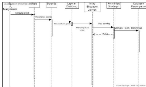
Gambar 6. Sequence Diagram Masyarakat
