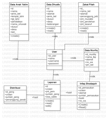
Gambar 7. Class Diagram System
