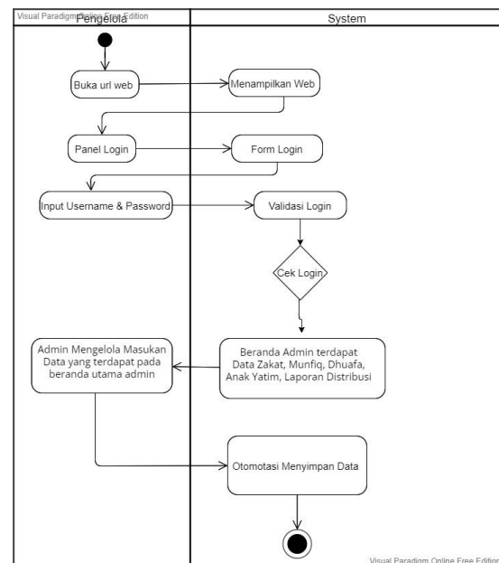
Gambar 3. Activity Diagram Pengelola
